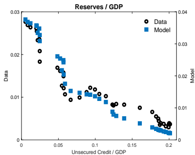
Figure 3: In-sample Fit: 1968-2007
