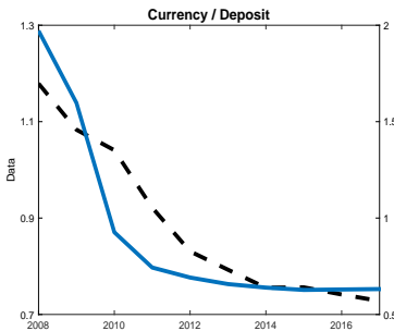
Figure 4: Out-of-sample Fit: 2008-2017
